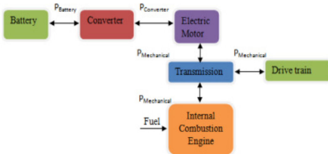
Fig. 2 Power flow of parallel HEV
